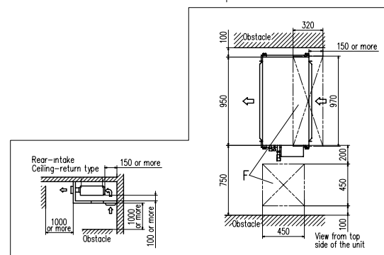
Space for installation and service
