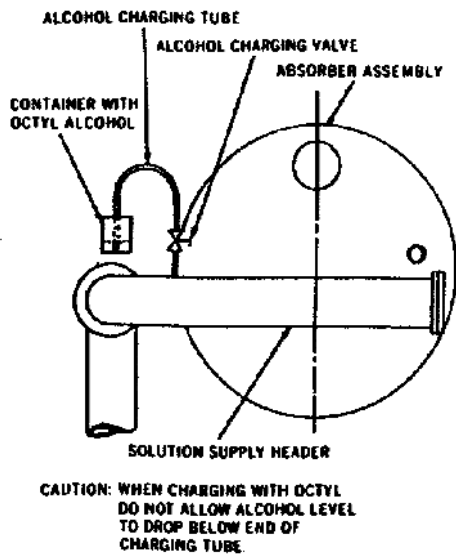
Figure 35. Octyl alcohol charging.
