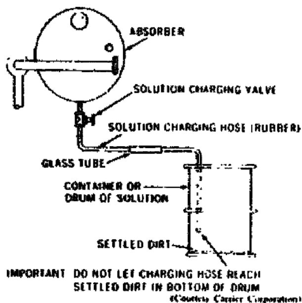
Figure 40. Solution charging.
