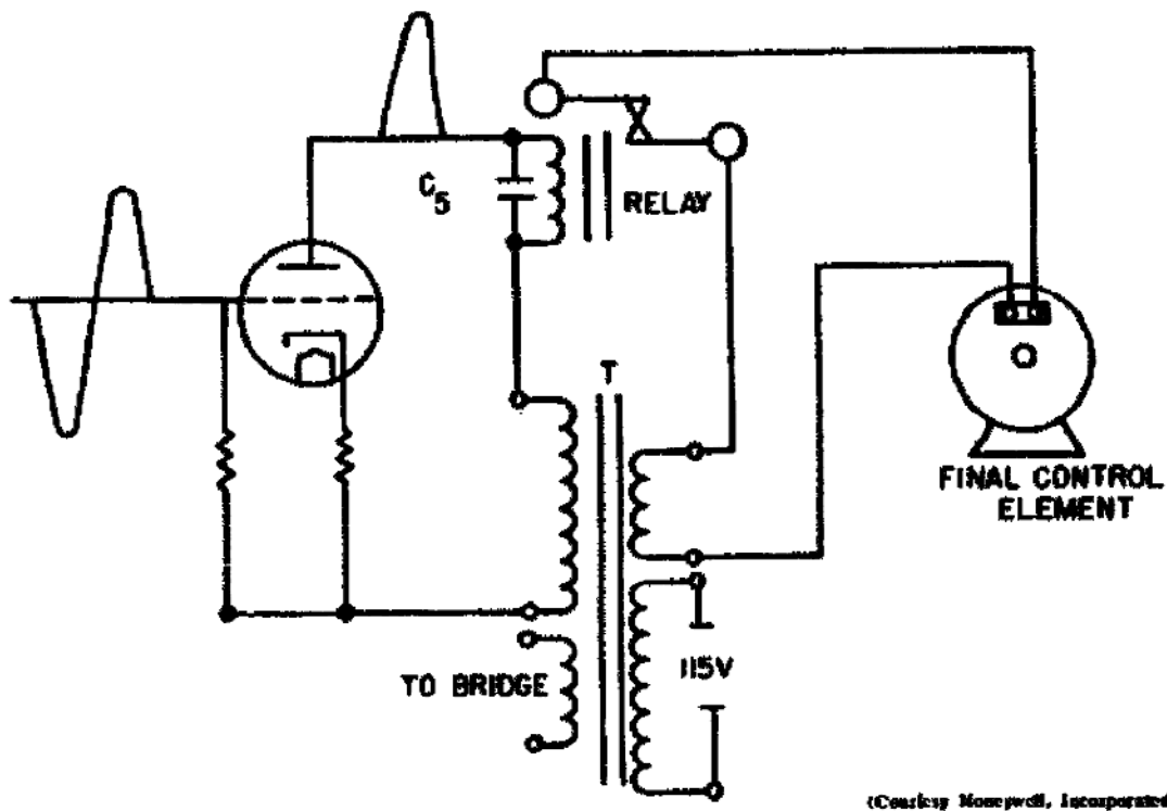
Figure 130. Discriminator circuit.
