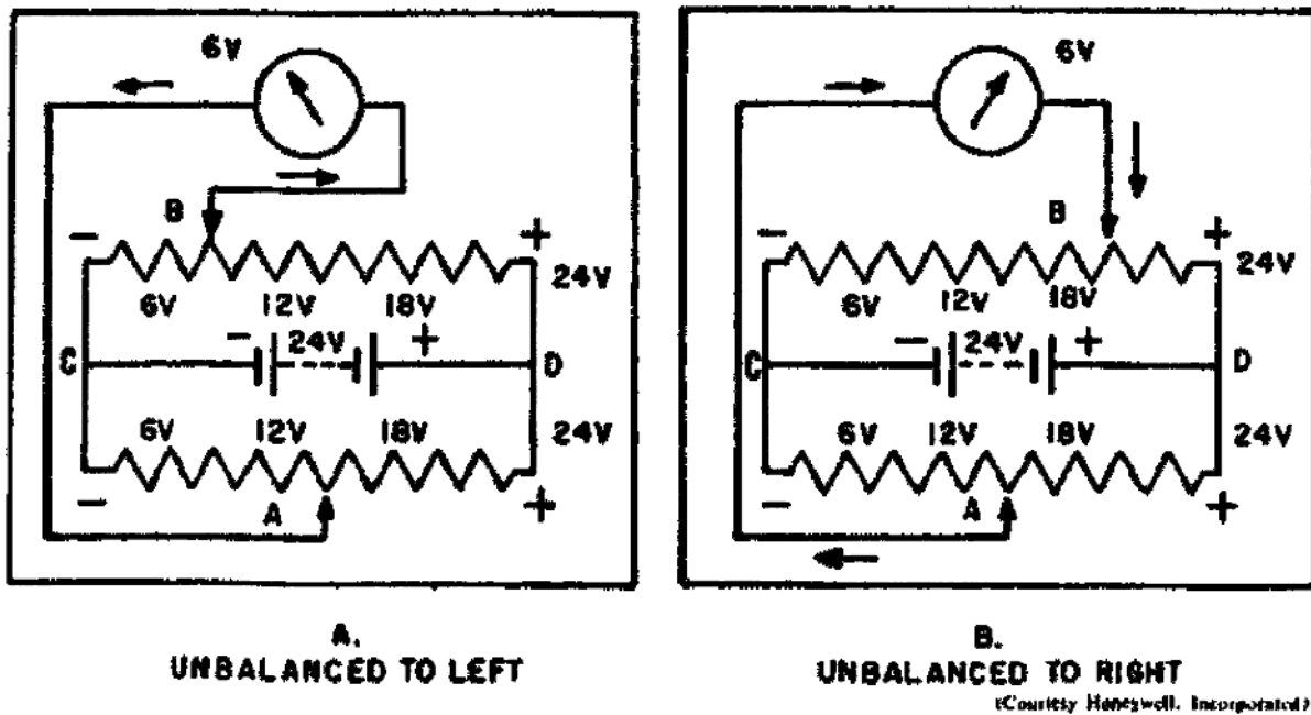
Figure 125. Simple bridge.
