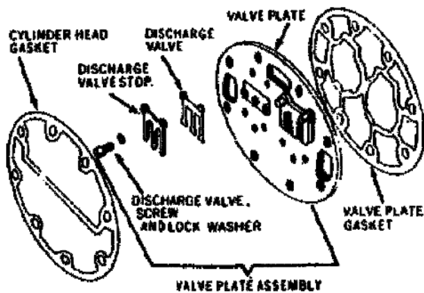
Figure 21. Valve plate assembly.
