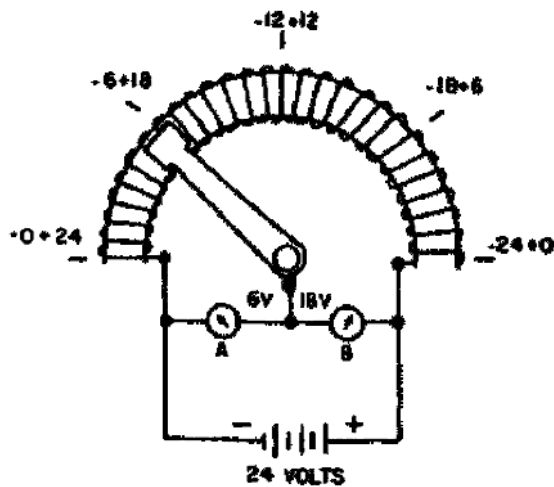
Figure 124. Potentiometer.
