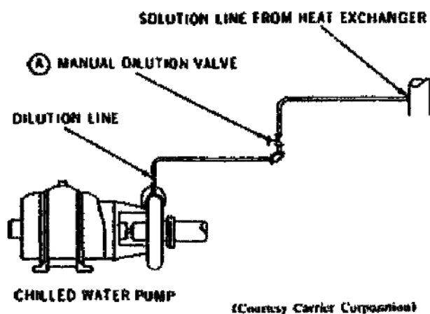
Figure 37. Manual dilution.
