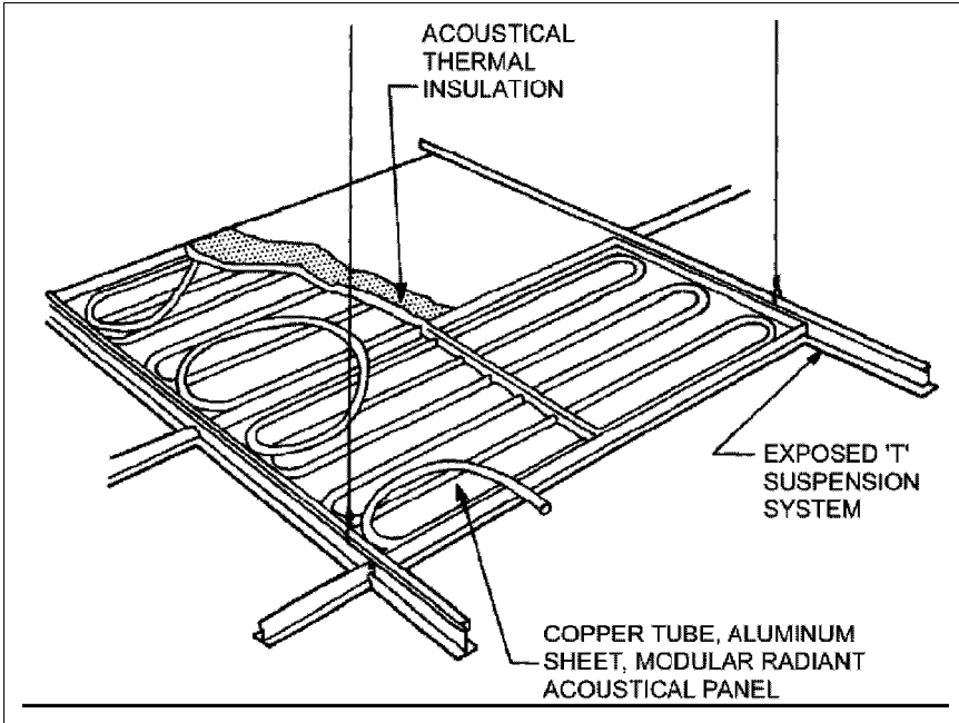
Figure 8-5 Example of Ceiling Radiant Panels
