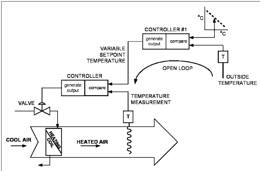
Figure 11-2 Open and Closed Control Loops
