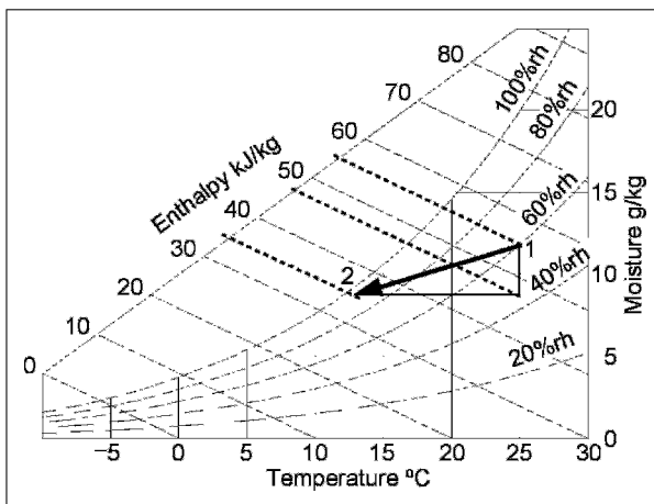
Figure 2-9 Psychrometric Chart—Cooling Across a Wet Cooling Coil
