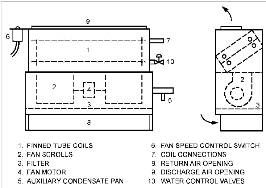
Figure 8-6 Typical Fan-Coil Unit
