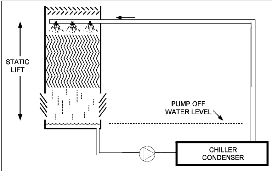
Figure 9-14 Open Water Circuit
