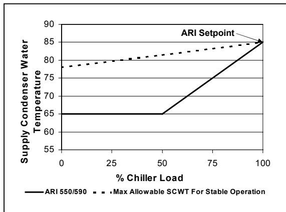
Figure 19 – Chiller Performance with Minimum Setpoint
