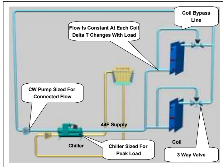
Figure 24 - Three-way Valves
