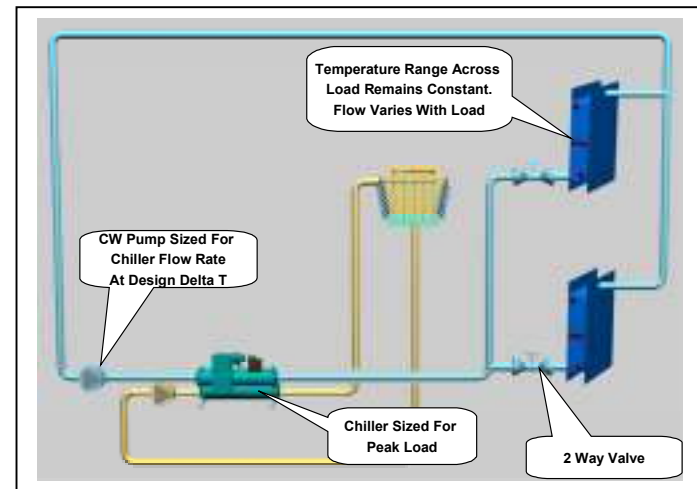
Figure 25 - Two-Way Valves
