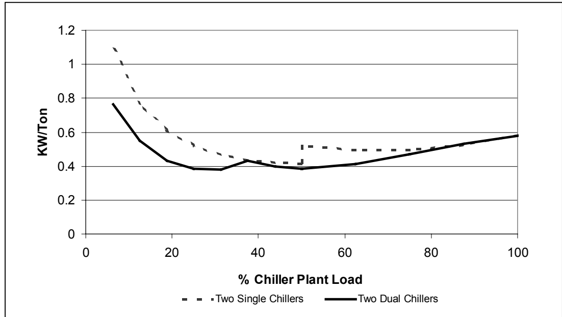
Figure 32 - Chiller Performance Vs. Plant Load
