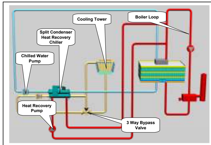
Figure 62 - Split Condenser Type Heat Recovery
