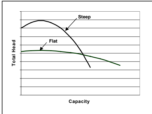
Figure 10 - Pump Curve Profiles
