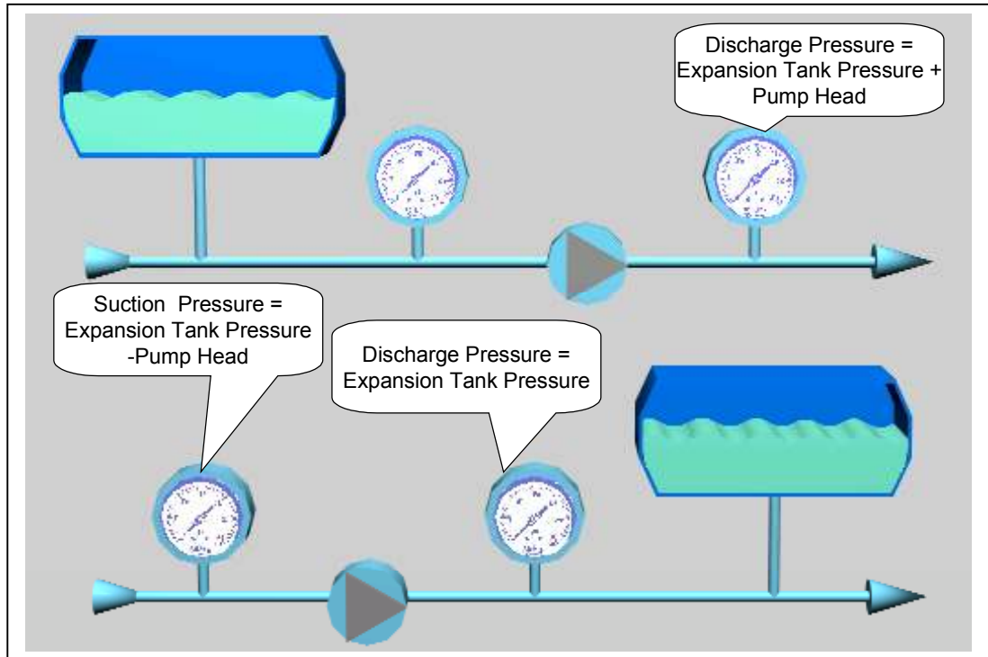
Figure 5 - Expansion Tank Location
