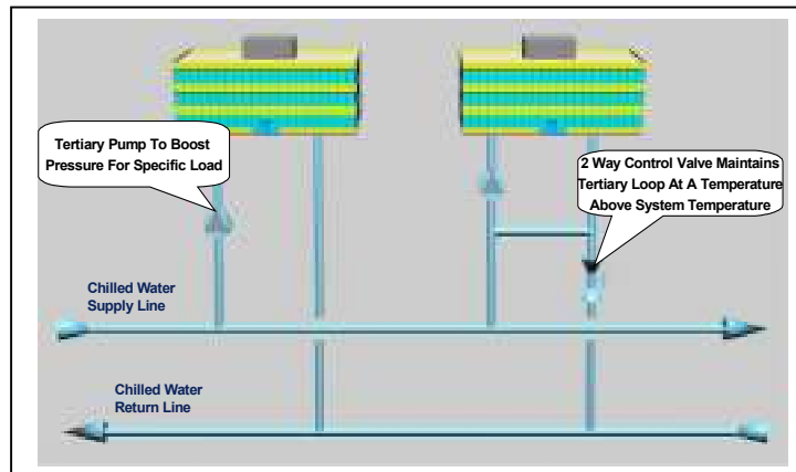
Figure 50 - Tertiary Pumping
