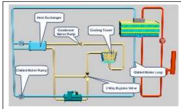
Figure 56 – Free Cooling with Tertiary Loop
