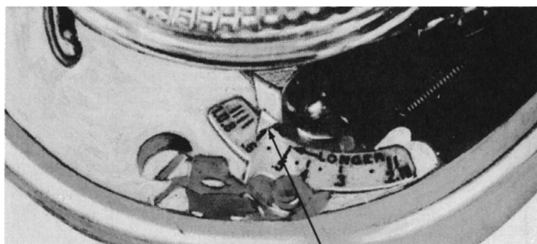
HEAT-ANTICIPATOR ADJUSTMENT
