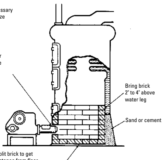
Figure 16-7 Combustion chamber for an older cast-iron boiler.
