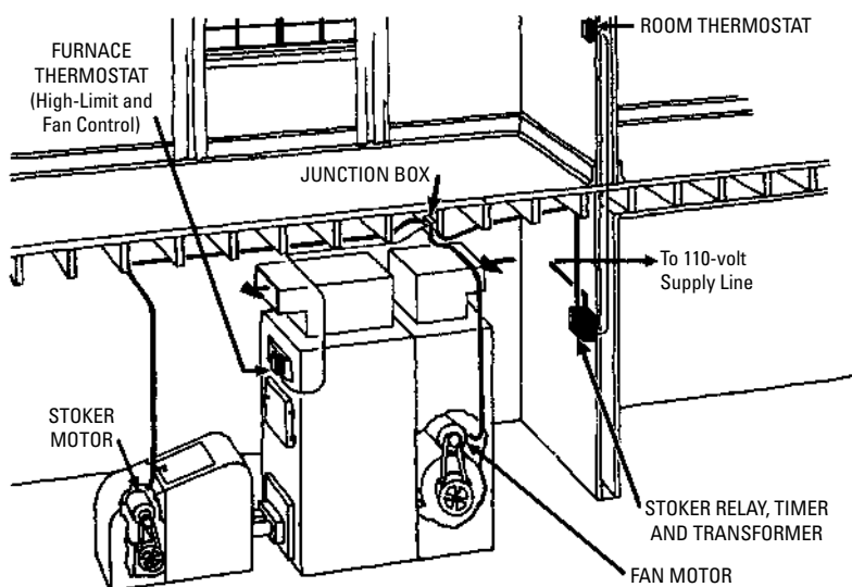
Figure 13-11 Automatic controls for a coal-fired furnace fed by a stoker. (Courtesy U.S. Department of Agriculture)
