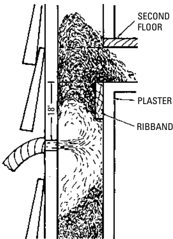
Figure 3-10 Blown-in insulation.
