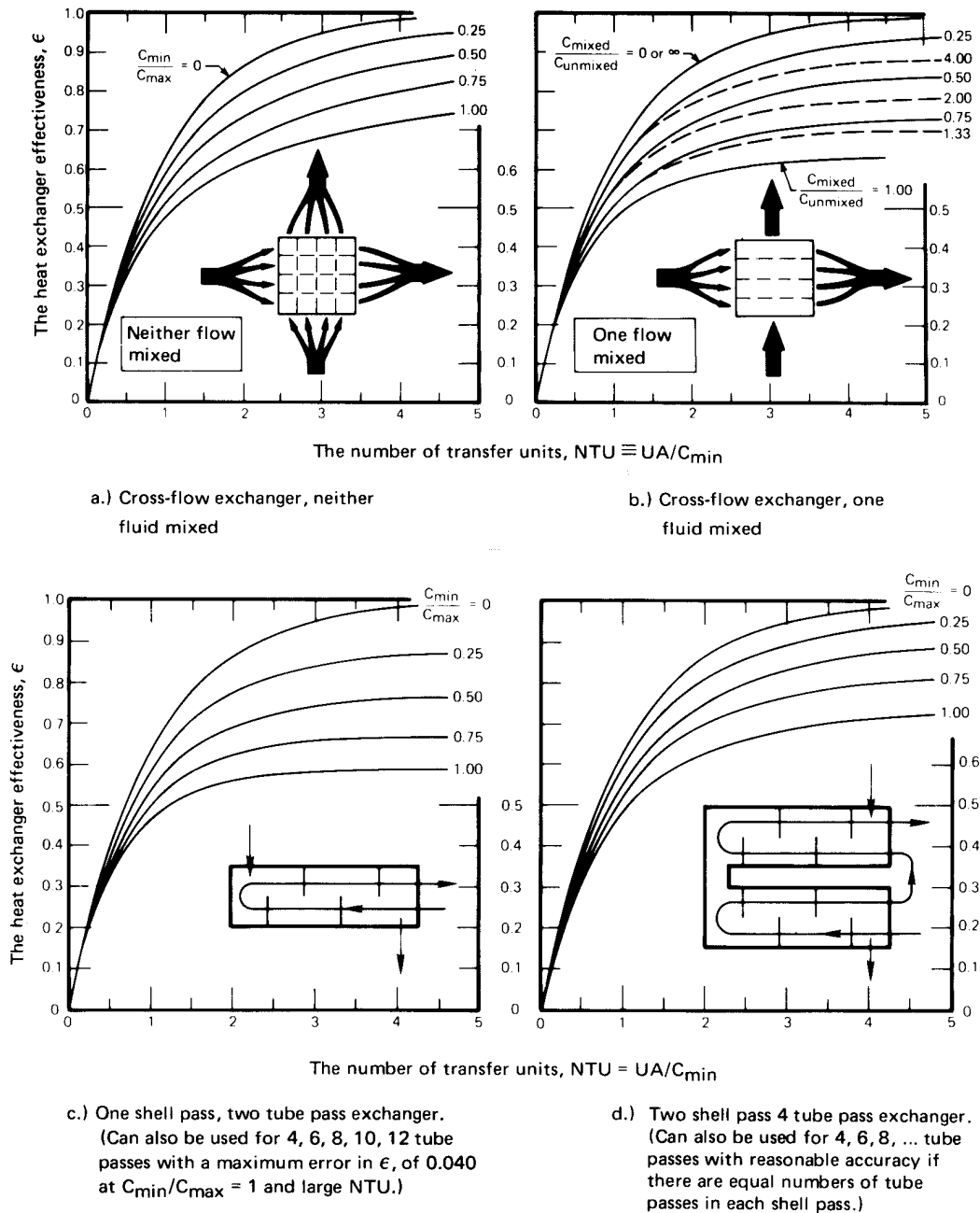
Figure 3.17 The effectiveness of some other heat exchanger configurations. (Data provided by A.D. Kraus.)
